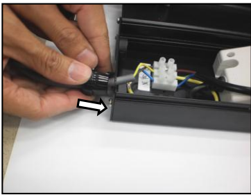
Step 3 : Attach back the cable bush with driver box.
