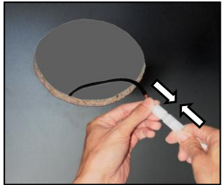
Step 4 : Connect the (male) connector from the transformer box to (female) connector from the lamp frame.
