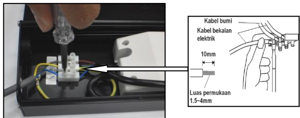
Step 2 : Insert supply cable into the driver box and connect to the prepared terminal block.
