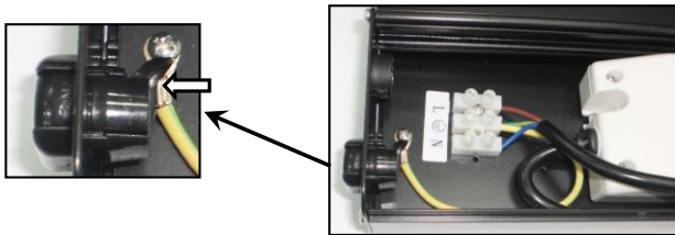
Step 1 : Push the pin inside the driver box to detach cable bush.
