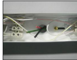
Step 5: Tie the fixture on ceiling after supply wire insert inside supply hole.
