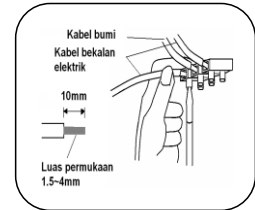
Step 6: Connect the supply wire in the provided connector.
