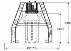
Drawing for PVRD 601 c/w PLCE Holder
