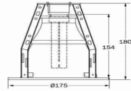
Drawing for PVRD 601 c/w PLC Holder
